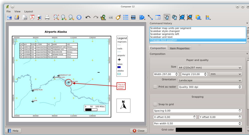
Рис. 18.20: Print Composer with map view, legend, scalebar, coordinates and text added 🐧
