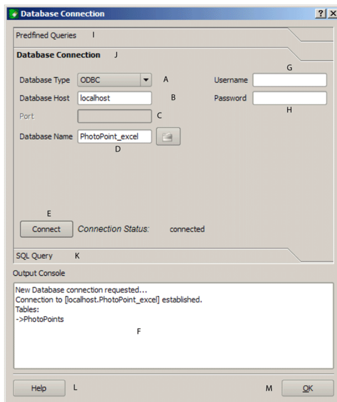
Рис. 19.12: The eVis Database connection window
